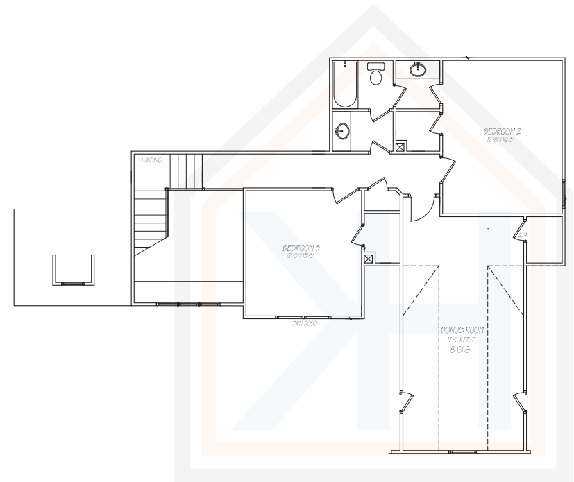
Bonus Floor Plan
